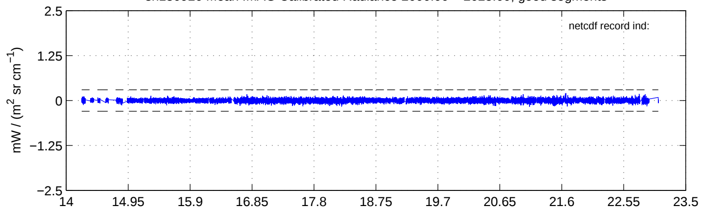
sh130926 Mean IMAG Calibrated Radiance 2000.00 – 2025.00, good segments
