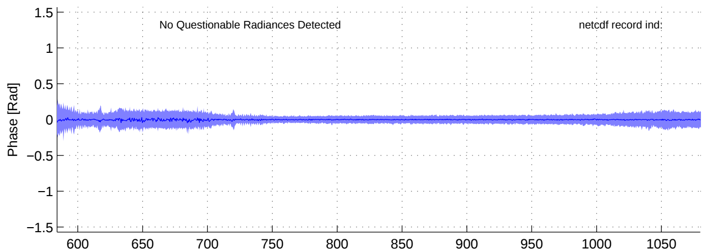
sh130926, PHASE(LW) Radiances included in shis_130926_sci_lw.nc BLUE = OK (meaned by seg); RED = significant imaginary content
