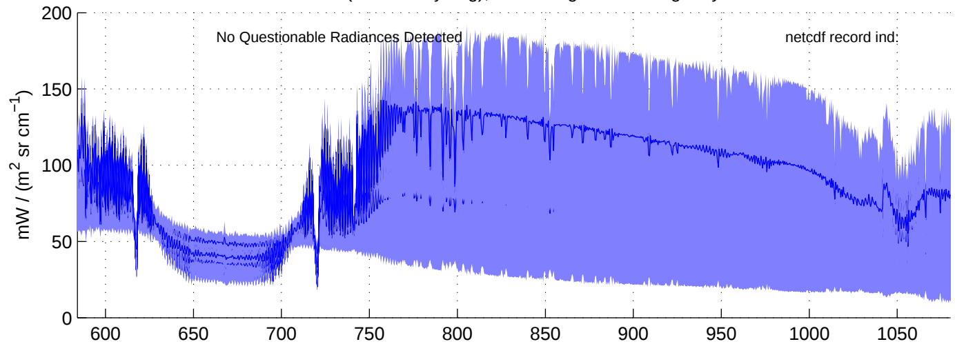
sh130926, REAL(LW) Radiances included in shis_130926_sci_lw.nc BLUE = OK (meaned by seg); RED = significant imaginary content
