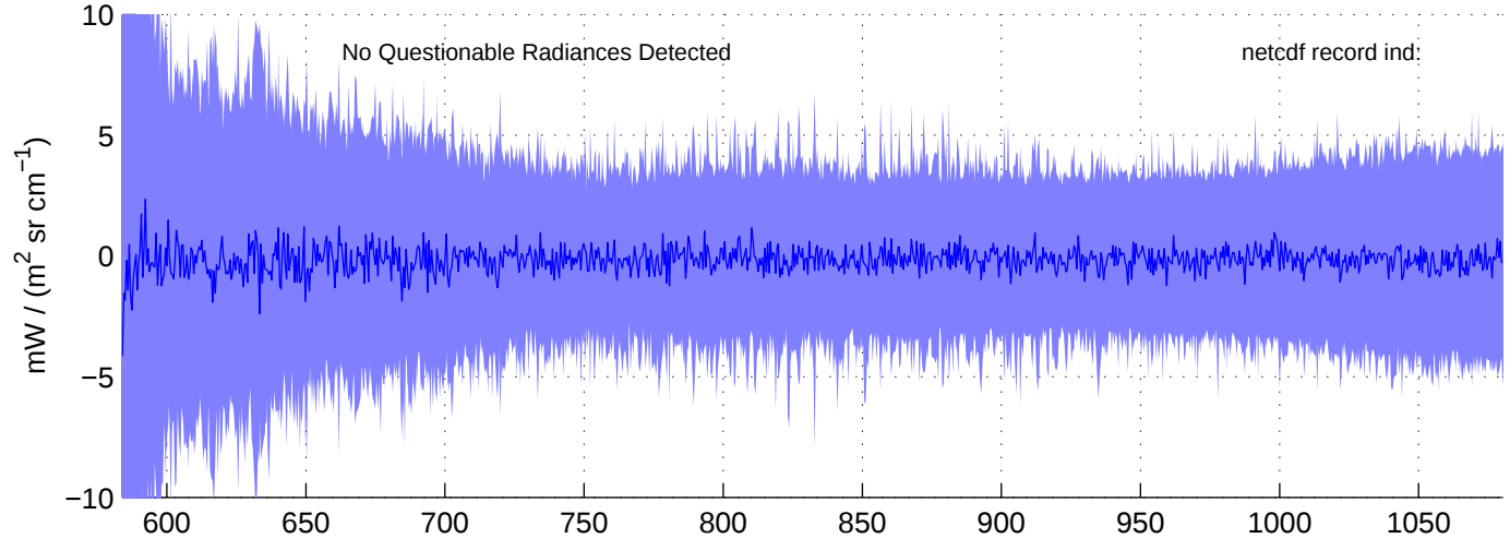
sh130926, Questionable (IMAG) LW Radiances included in shis_130926_sci_lw.nc BLUE = OK (meaned by seg); RED = significant imaginary content
