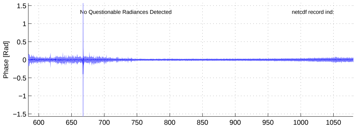
sh130917, PHASE(LW) Radiances included in shis_130917_sci_lw.nc BLUE = OK (meaned by seg); RED = significant imaginary content
