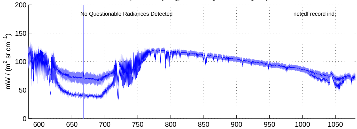
sh130917, REAL(LW) Radiances included in shis_130917_sci_lw.nc BLUE = OK (meaned by seg); RED = significant imaginary content
