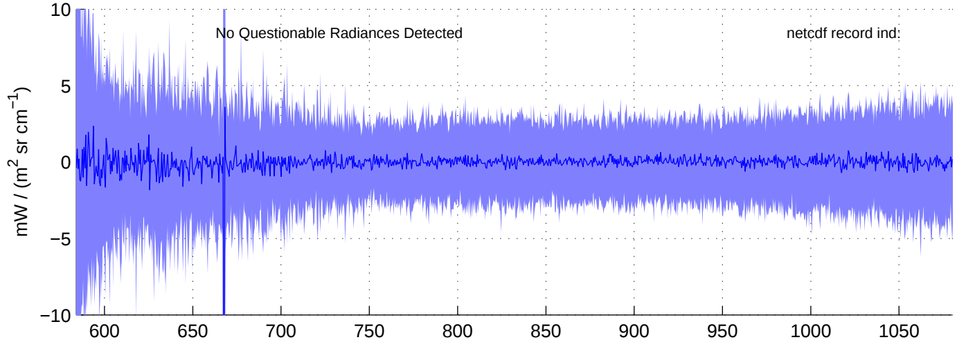
sh130917, Questionable (IMAG) LW Radiances included in shis_130917_sci_lw.nc BLUE = OK (meaned by seg); RED = significant imaginary content
