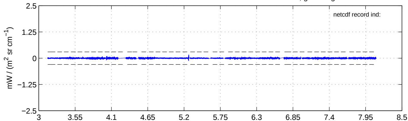
sh130908 Mean IMAG Calibrated Radiance 2000.00 – 2025.00, good segments
