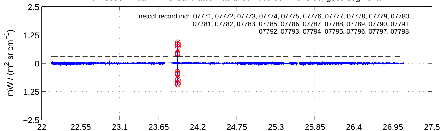
sh130907 Mean IMAG Calibrated Radiance 2000.00 – 2025.00, good segments
