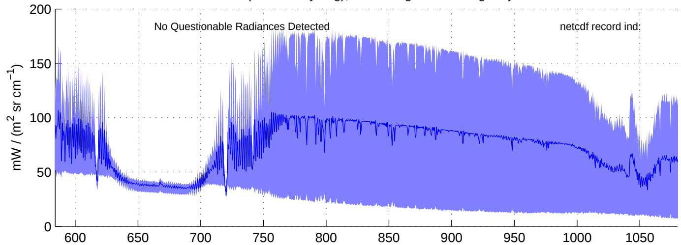
sh130908, REAL(LW) Radiances included in shis_130908_sci_lw.nc BLUE = OK (meaned by seg); RED = significant imaginary content
