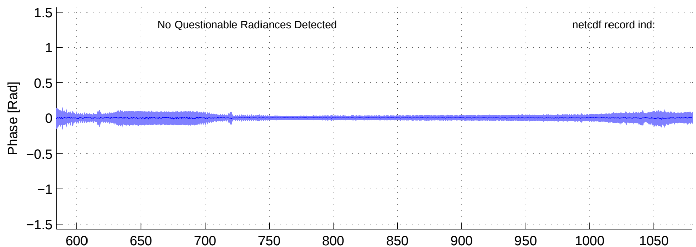
sh130908, PHASE(LW) Radiances included in shis_130908_sci_lw.nc BLUE = OK (meaned by seg); RED = significant imaginary content
