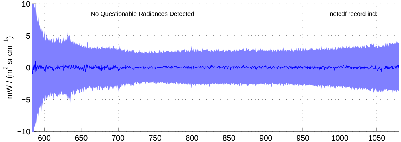
sh130908, Questionable (IMAG) LW Radiances included in shis_130908_sci_lw.nc BLUE = OK (meaned by seg); RED = significant imaginary content
