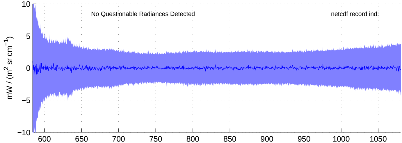
sh130907, Questionable (IMAG) LW Radiances included in shis_130907_sci_lw.nc BLUE = OK (meaned by seg); RED = significant imaginary content
