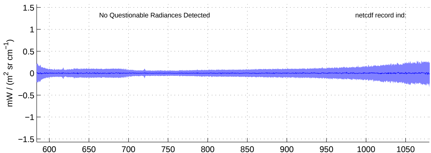
sh130907, PHASE(LW) Radiances included in shis_130907_sci_lw.nc BLUE = OK (meaned by seg); RED = significant imaginary content
