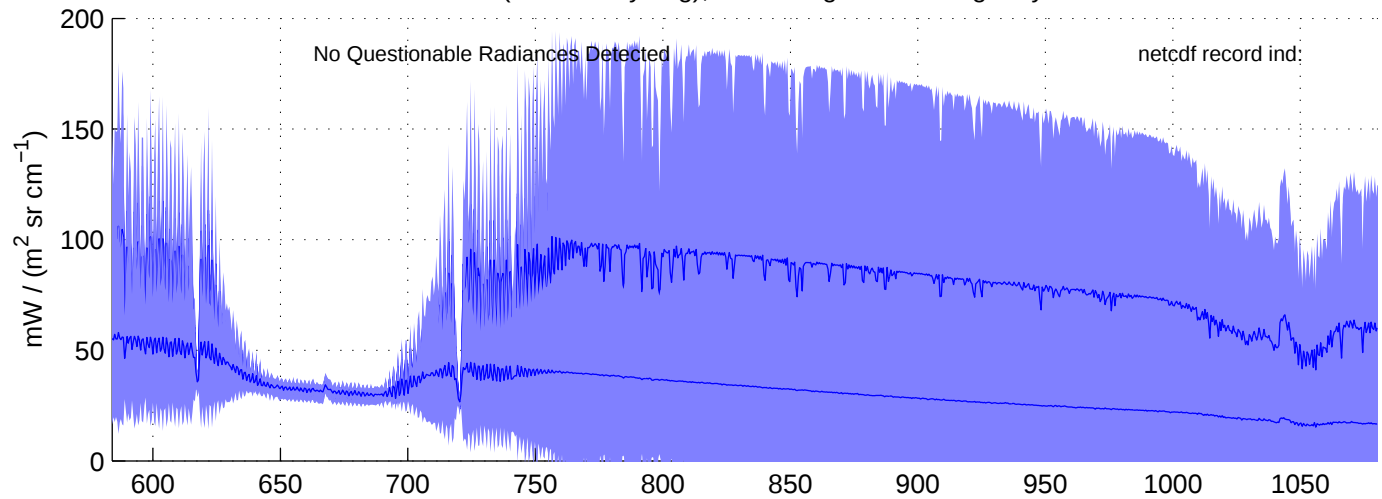
sh130907, REAL(LW) Radiances included in shis_130907_sci_lw.nc BLUE = OK (meaned by seg); RED = significant imaginary content
