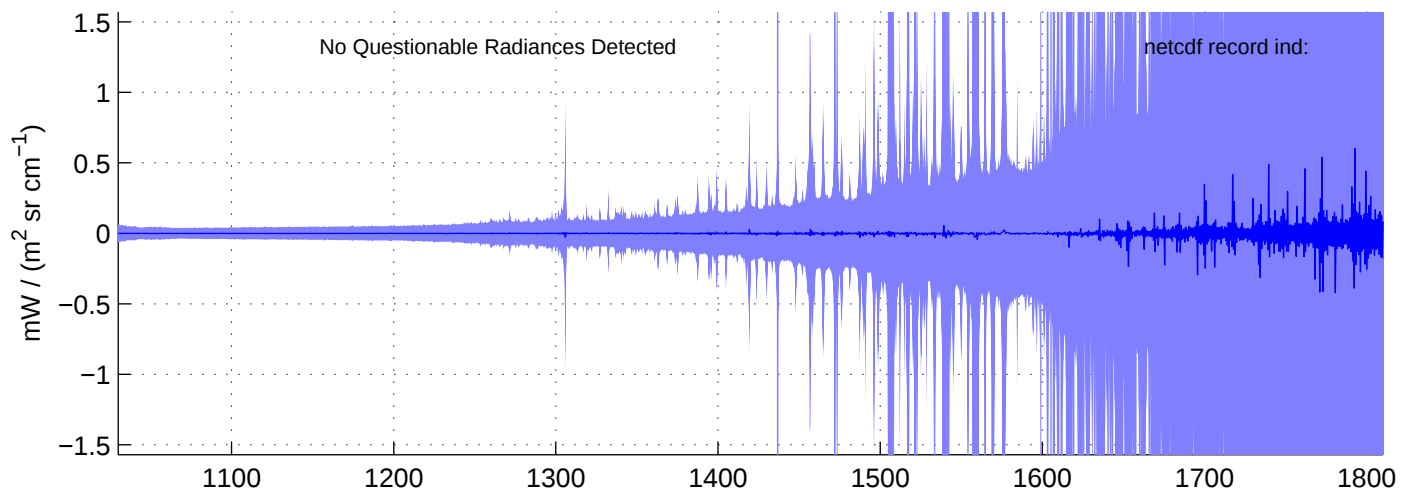
sh130907, PHASE(MW) Radiances included in shis_130907_sci_mw.nc BLUE = OK (meaned by seg); RED = significant imaginary content
