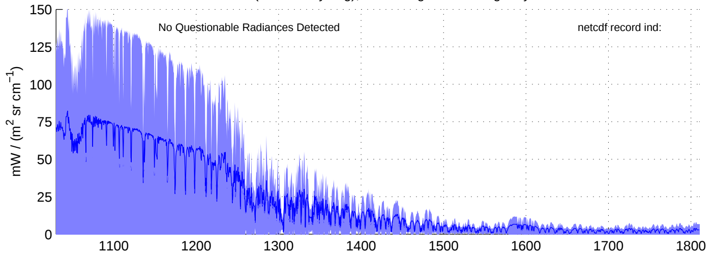
sh130907, REAL(MW) Radiances included in shis_130907_sci_mw.nc BLUE = OK (meaned by seg); RED = significant imaginary content
