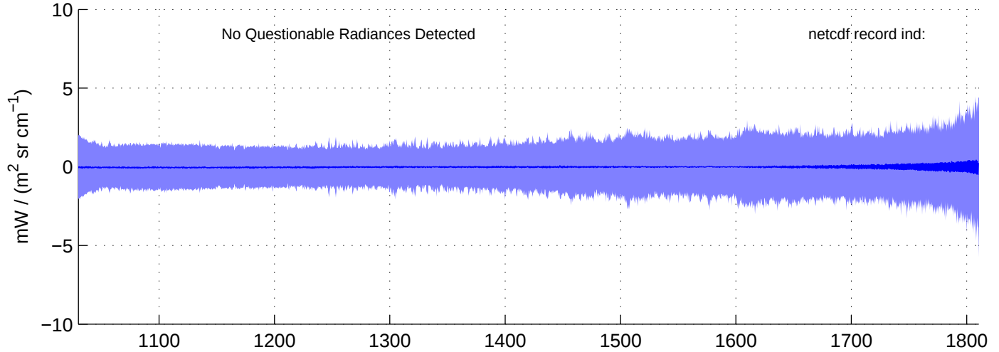
sh130907, IMAG(MW) Radiances included in shis_130907_sci_mw.nc BLUE = OK (meaned by seg); RED = significant imaginary content
