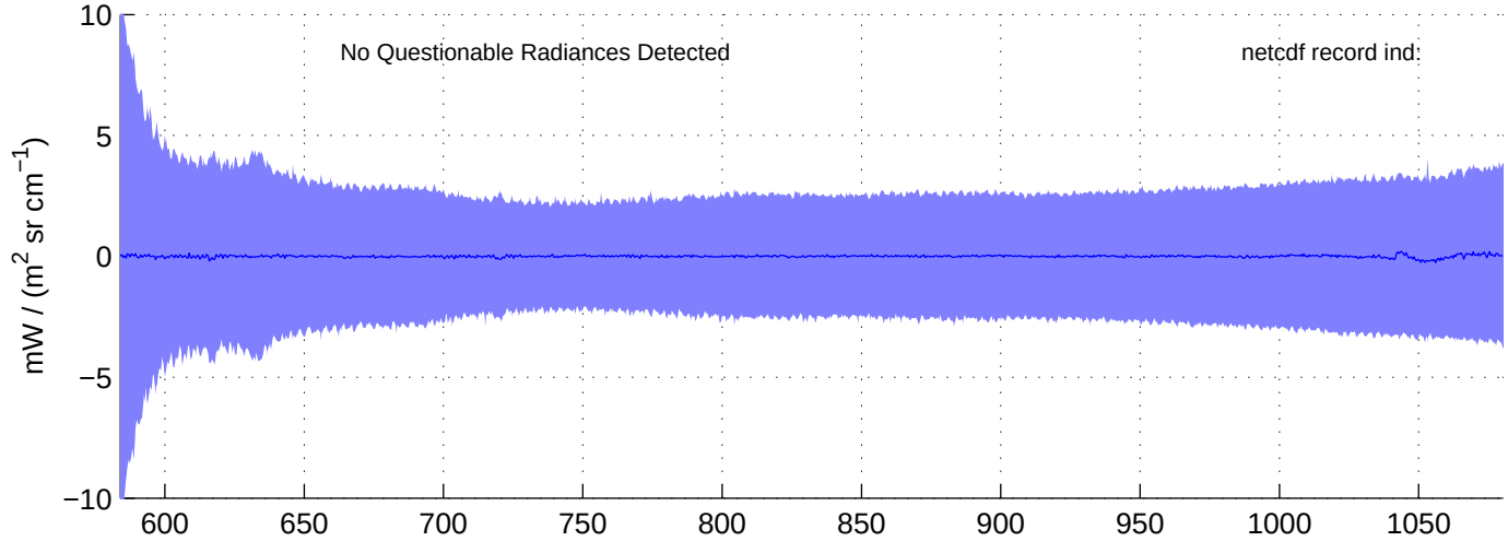
sh130825, Questionable (IMAG) LW Radiances included in shis_130825_sci_lw.nc BLUE = OK (meaned by seg); RED = significant imaginary content
