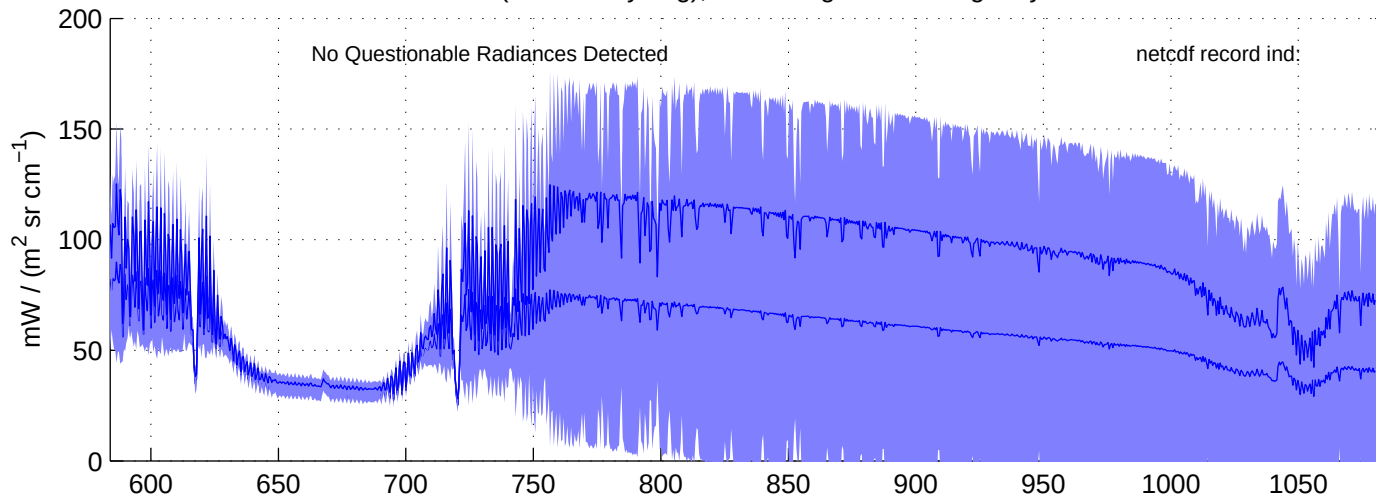
sh130825, REAL(LW) Radiances included in shis_130825_sci_lw.nc BLUE = OK (meaned by seg); RED = significant imaginary content
