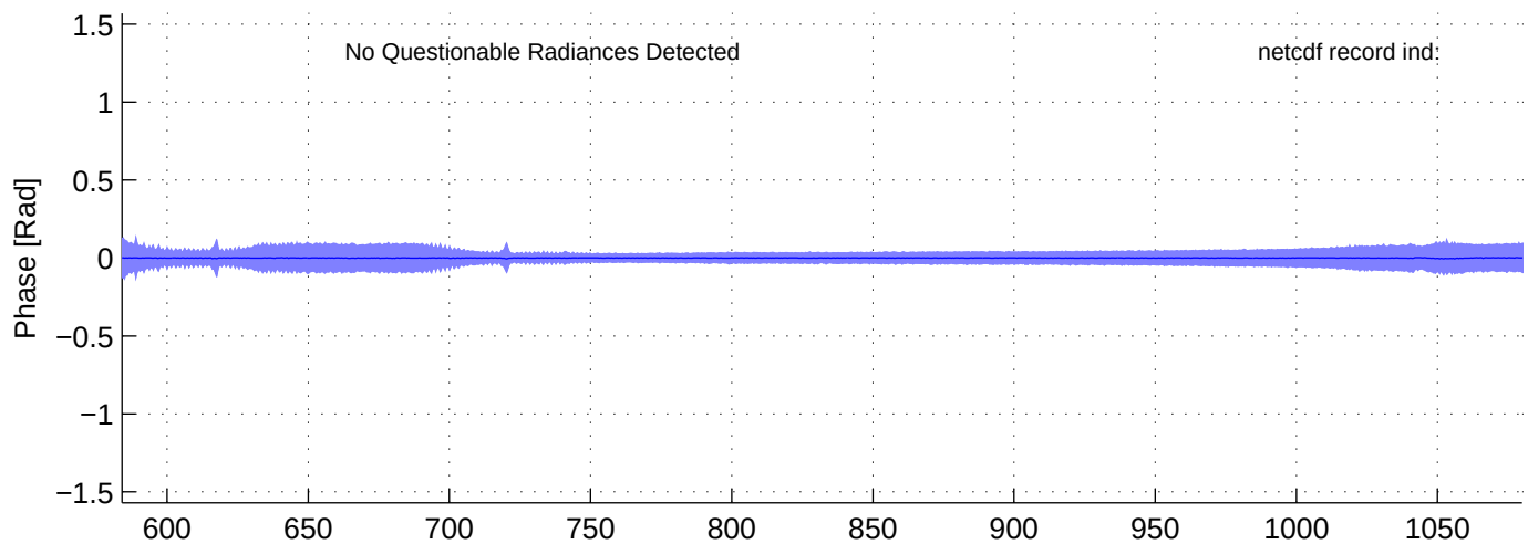
sh130825, PHASE(LW) Radiances included in shis_130825_sci_lw.nc BLUE = OK (meaned by seg); RED = significant imaginary content
