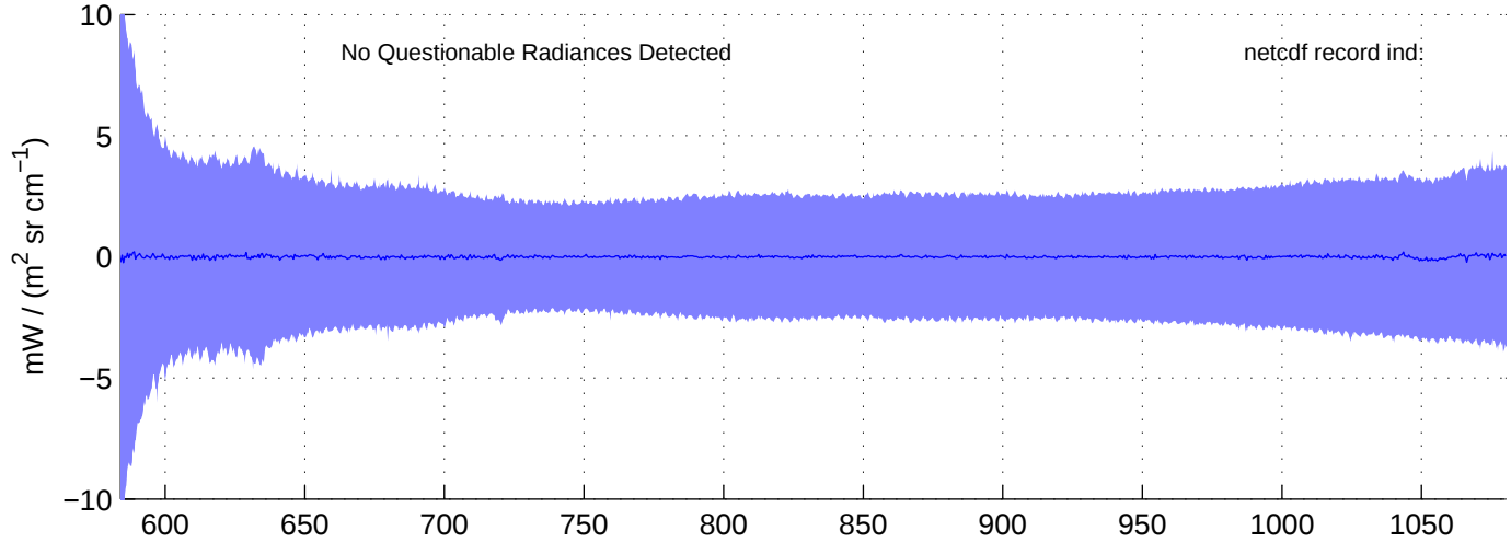
sh130824, Questionable (IMAG) LW Radiances included in shis_130824_sci_lw.nc BLUE = OK (meaned by seg); RED = significant imaginary content
