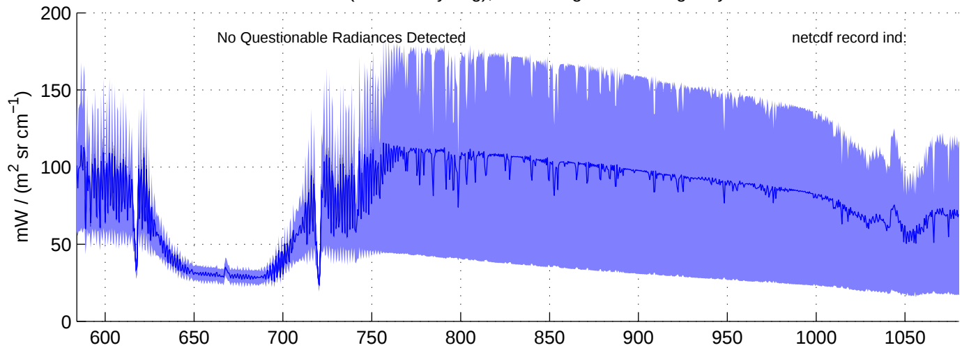
sh130824, REAL(LW) Radiances included in shis_130824_sci_lw.nc BLUE = OK (meaned by seg); RED = significant imaginary content
